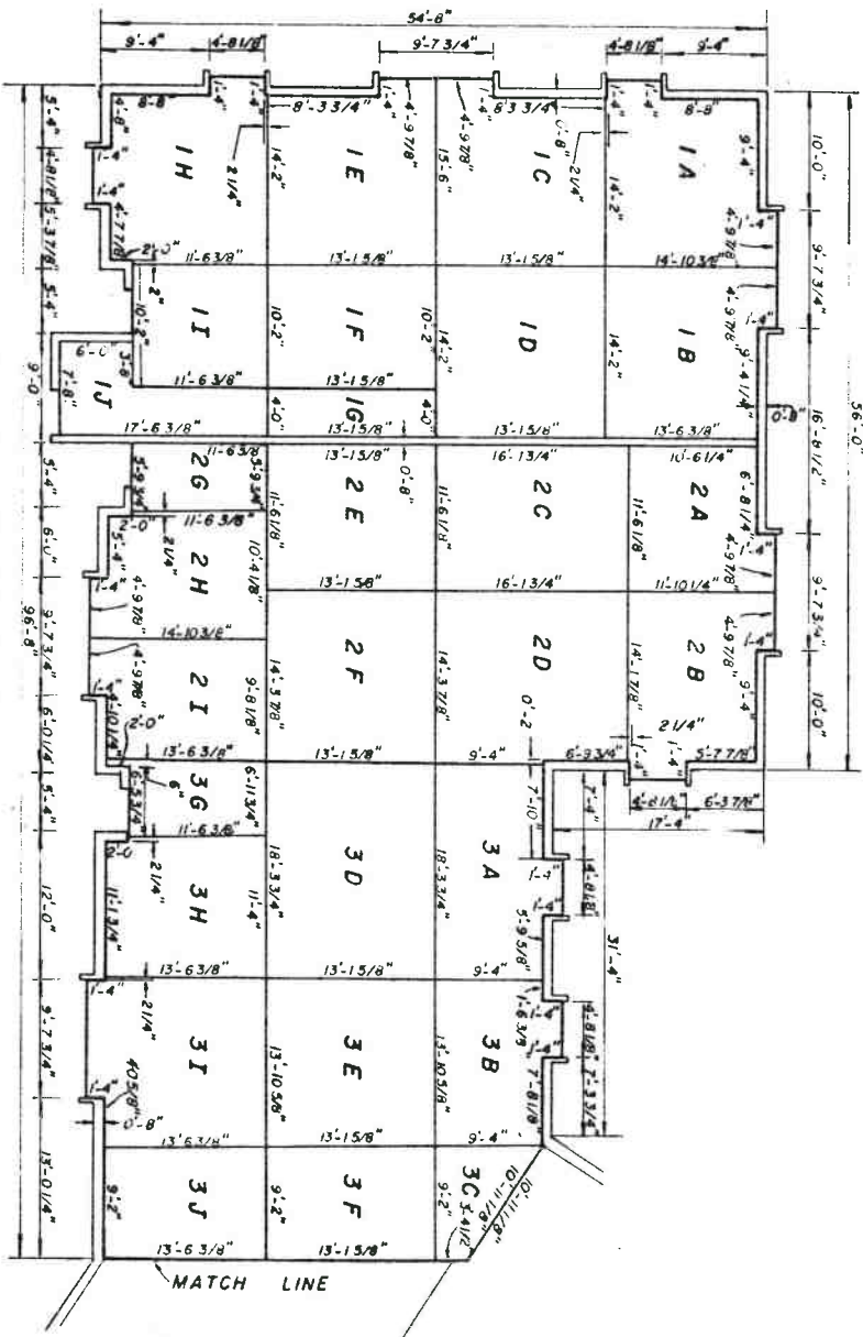
FIRST LEVEL FLOOR PLAN (BUILDING "D") FLOOR ELEV. *17.00 CEILING ELEV. *26.33
