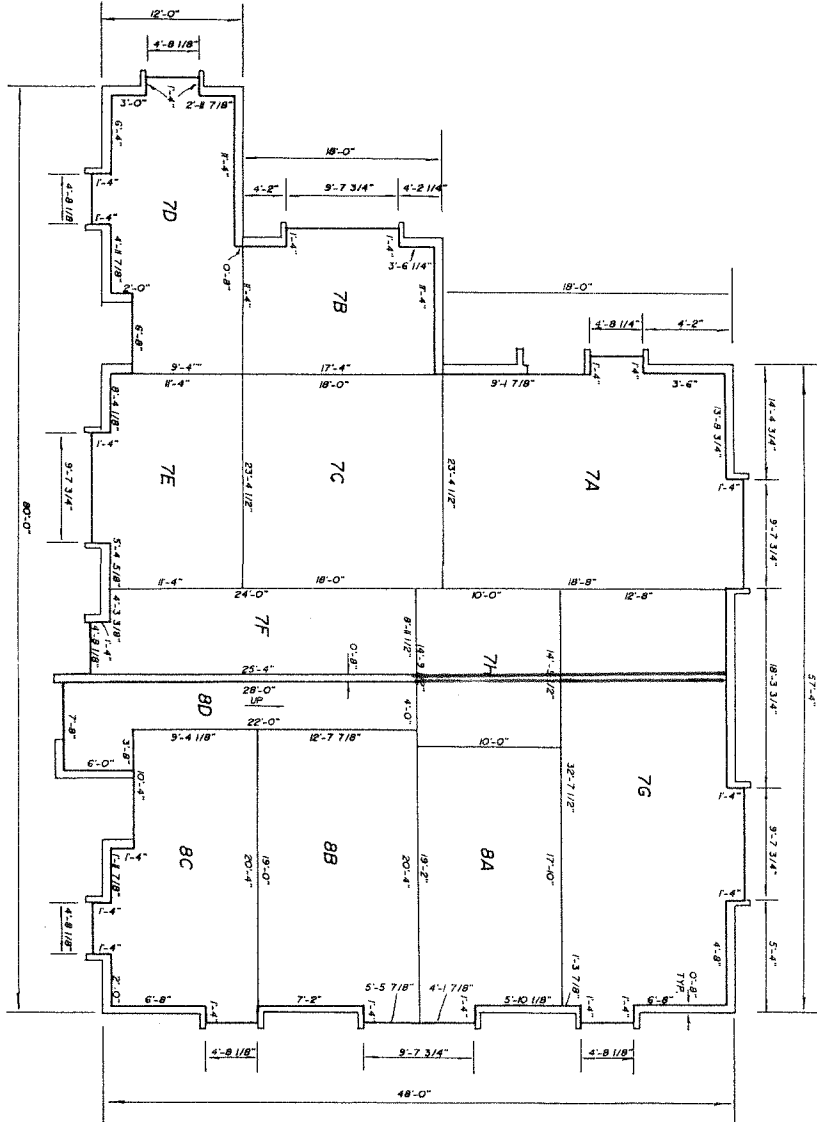
FIRST LEVEL FLOOR PLAN (BUILDING "E") FLOOR ELEV. +17.75; CEILING ELEV. +27.08
