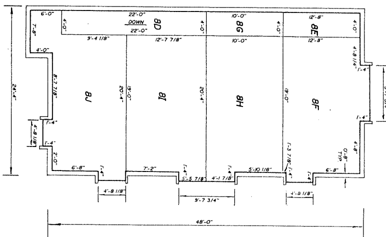
SECOND LEVEL FLOOR PLAN (BUILDING "E") FLOOR ELEV. +28.46' CEILING ELEV. +37.75'
